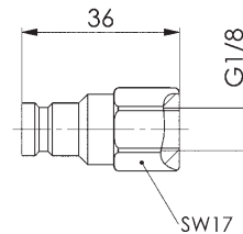
558043 Connector
